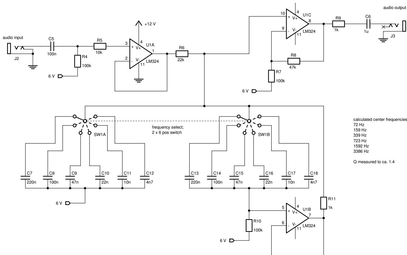
Bandpass filter (gyrator) filter section
